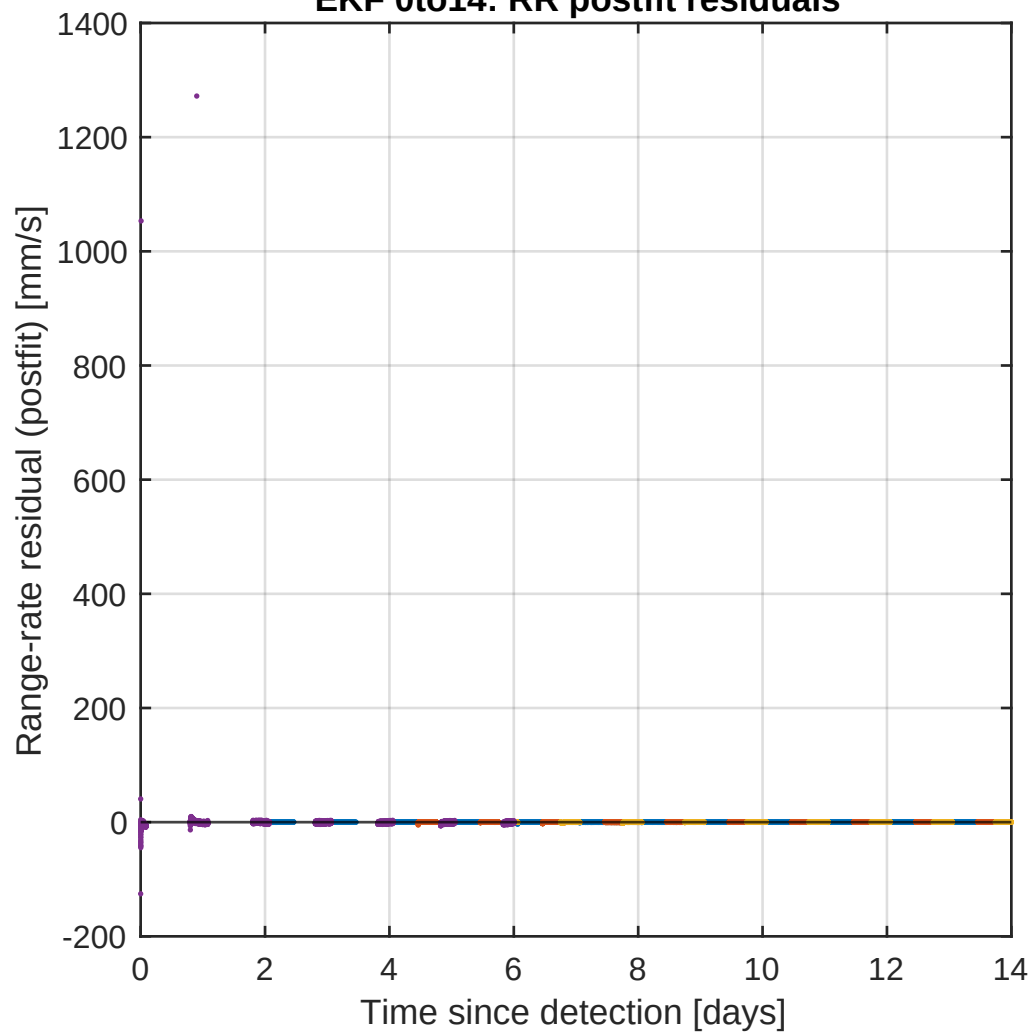
EKF 0to14: RR postfit residuals
